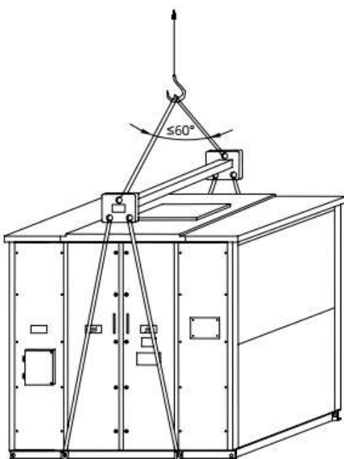
Handling transformer with enclosure
